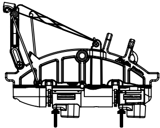
81499001 MD 180 SPINE ASSY INCLUDES SPROCKETS, GUARDS AND SHIFTERS
